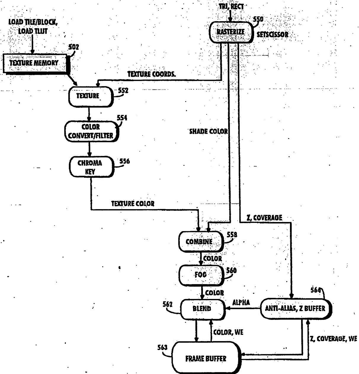
Fig. 18 DISPLAY PROCESSOR PROCESSING
